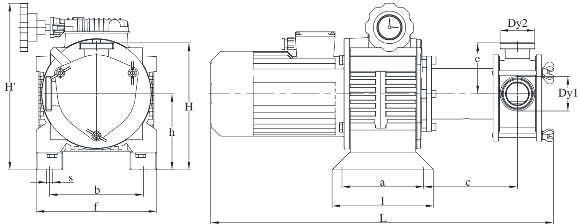
Dimensions, mm
